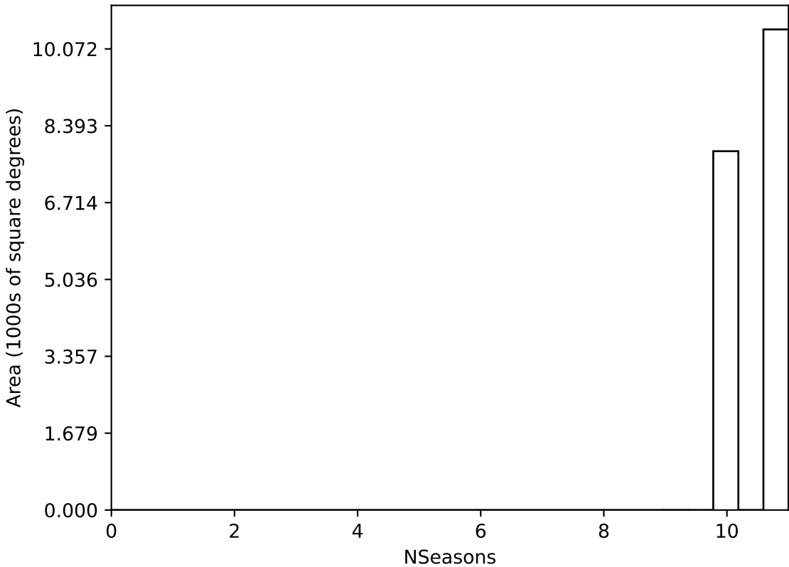
internal_u_expt38_nscale1.1v3.4_10yrs WFD all bands: NSeasons
