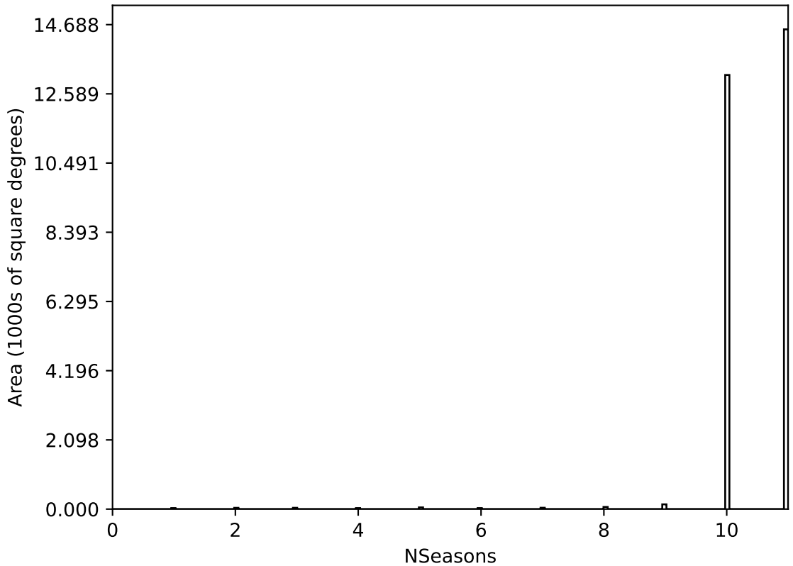
internal_u_expt38_nscale1.1v3.4_10yrs All sky all bands: NSeasons
