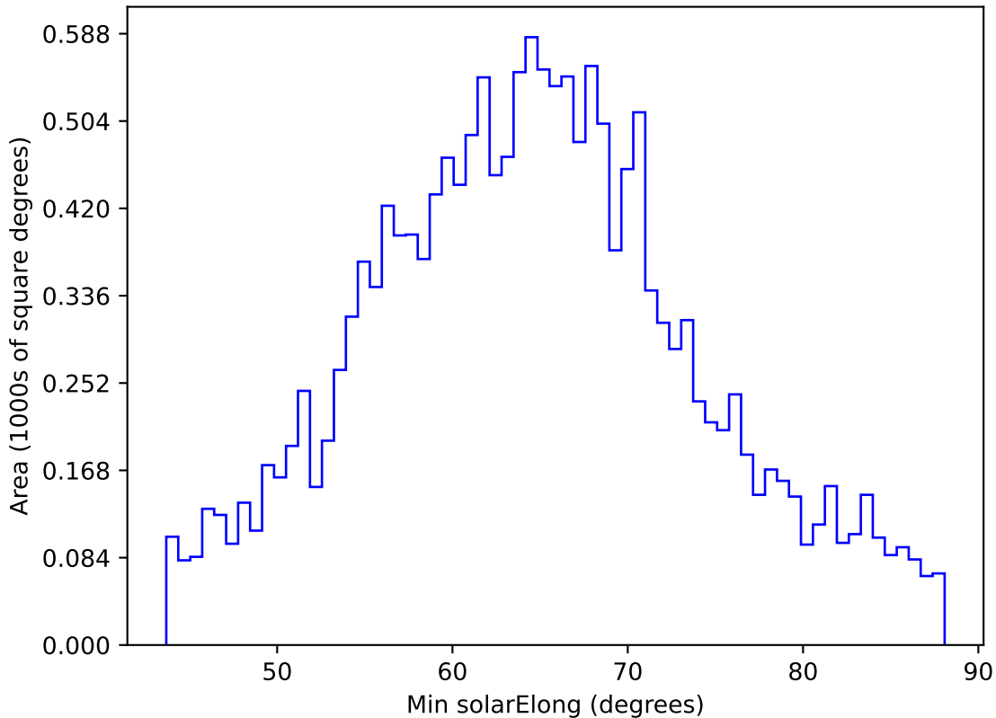
internal_u_expt38_nscale1.1v3.4_10yrs WFD y band: Min solarElong
