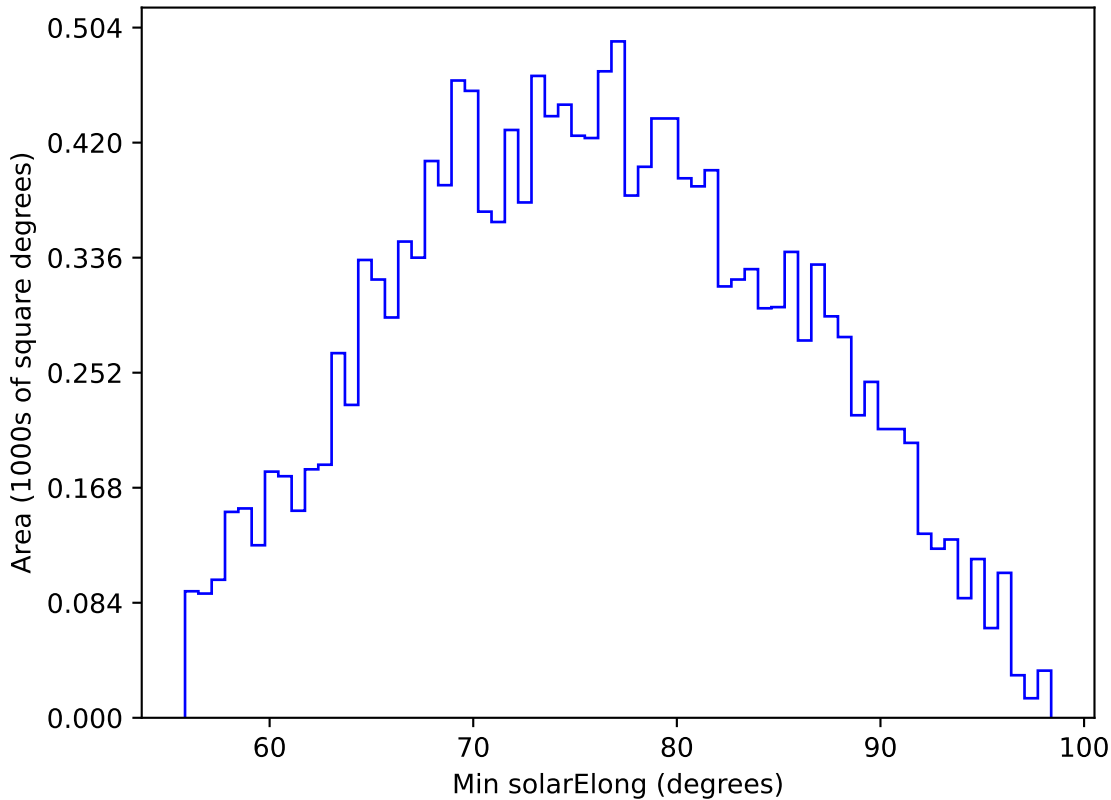
internal_u_expt38_nscale1.1v3.4_10yrs WFD u band: Min solarElong
