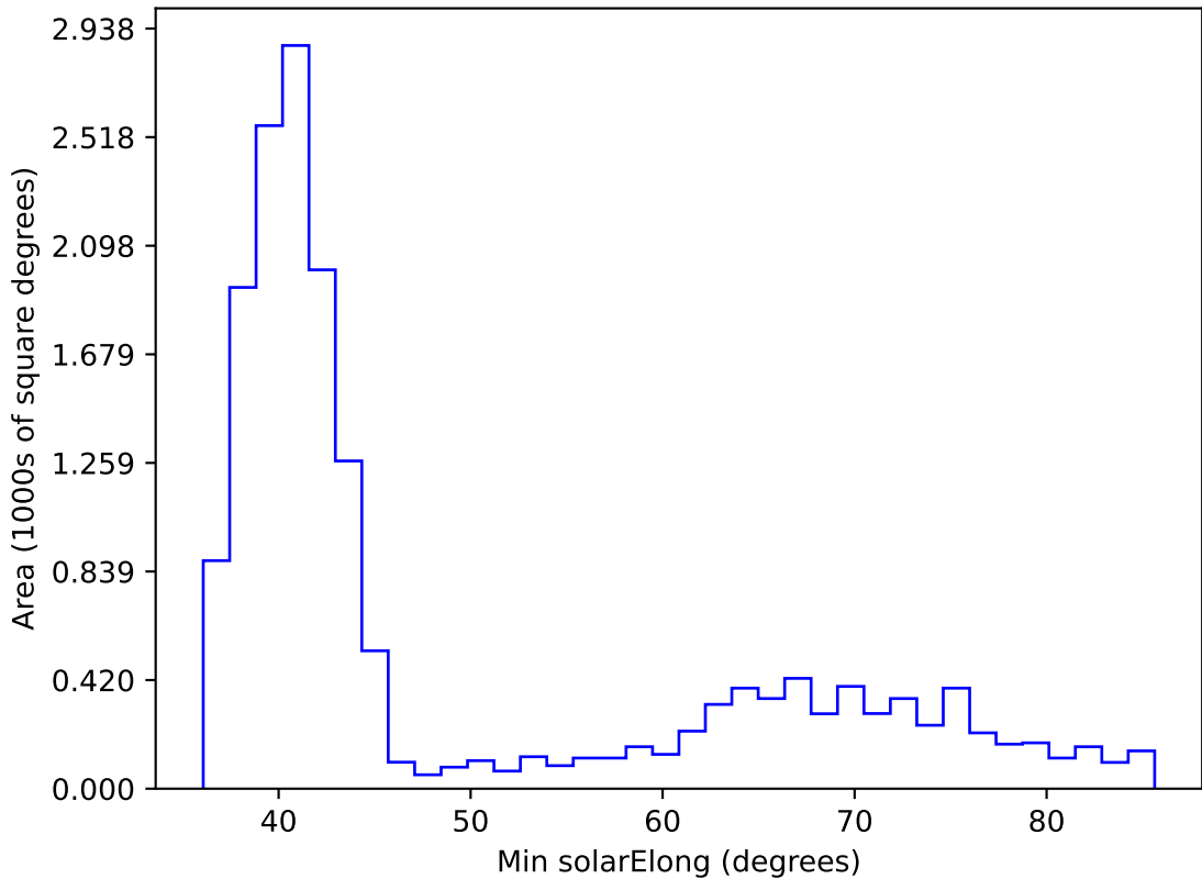
internal_u_expt38_nscale1.1v3.4_10yrs WFD i band: Min solarElong
