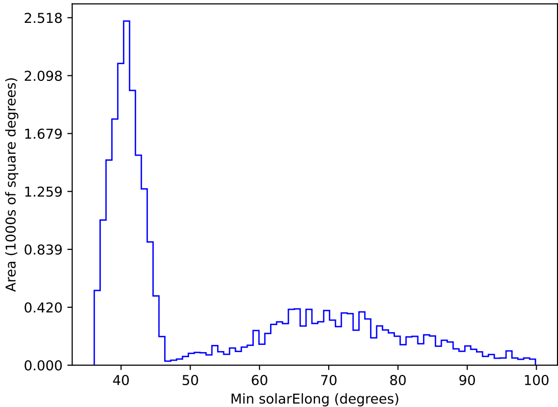
internal_u_expt38_nscale1.1v3.4_10yrs All sky i band: Min solarElong
