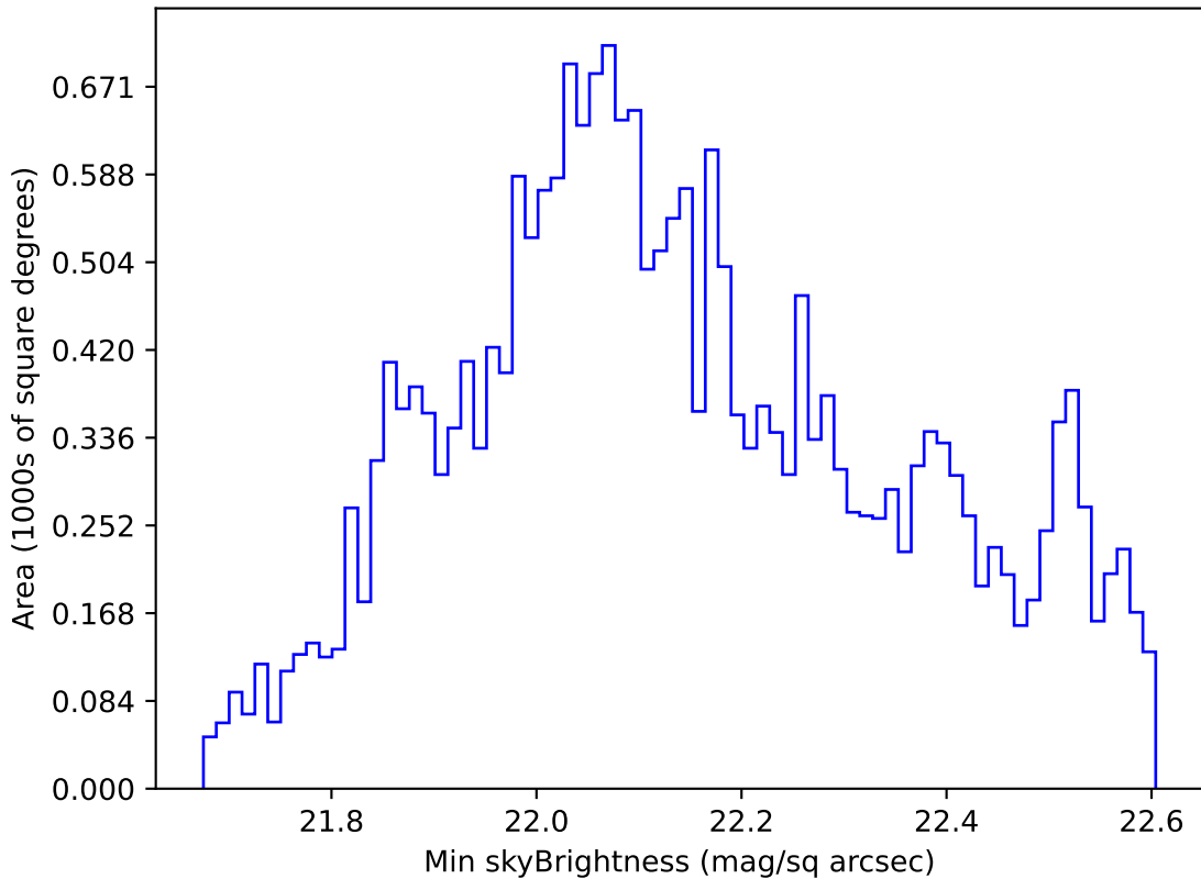
internal_u_expt38_nscale1.1v3.4_10yrs All sky u band: Min skyBrightness
