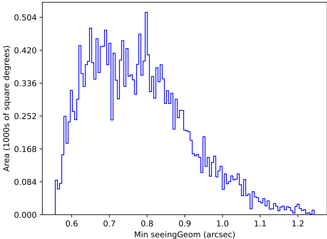
internal_u_expt38_nscale1.1v3.4_10yrs Yr 1 u band: Min seeingGeom
