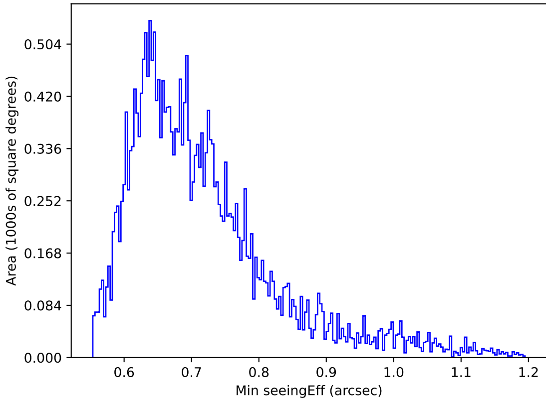
internal_u_expt38_nscale1.1v3.4_10yrs Yr 1 z band: Min seeingEff
