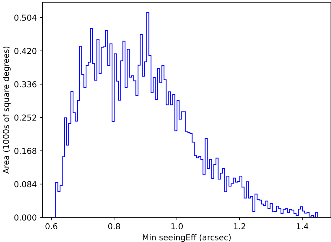
internal_u_expt38_nscale1.1v3.4_10yrs Yr 1 u band: Min seeingEff
