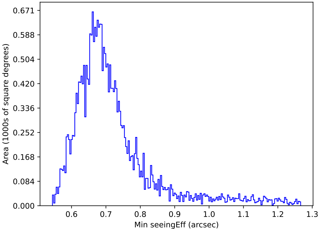
internal_u_expt38_nscale1.1v3.4_10yrs Yr 1 r band: Min seeingEff
