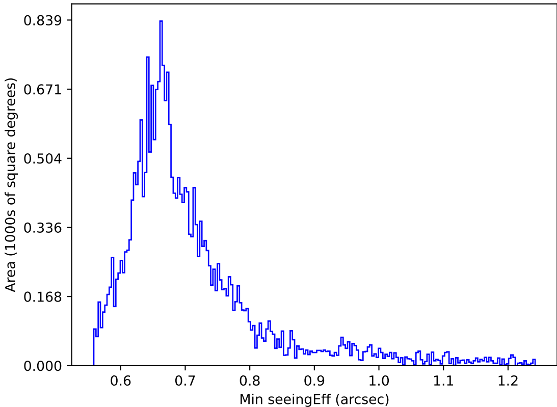
internal_u_expt38_nscale1.1v3.4_10yrs Yr 1 i band: Min seeingEff
