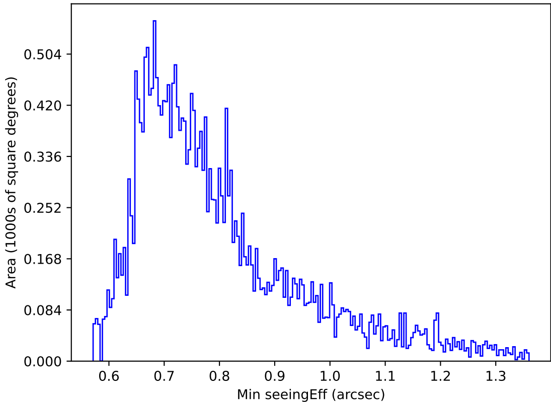
internal_u_expt38_nscale1.1v3.4_10yrs Yr 1 g band: Min seeingEff
