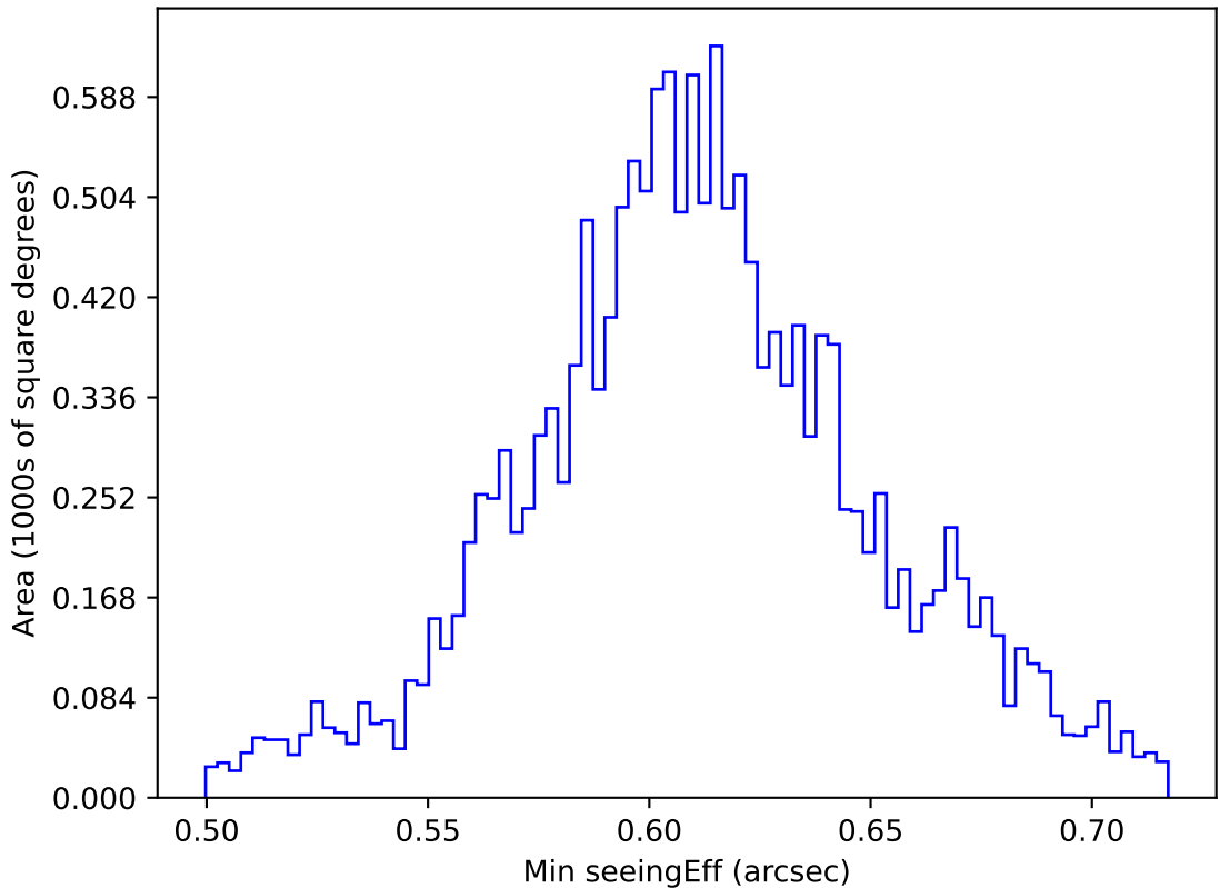
internal_u_expt38_nscale1.1v3.4_10yrs WFD z band: Min seeingEff
