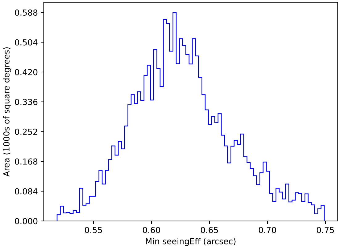
internal_u_expt38_nscale1.1v3.4_10yrs WFD y band: Min seeingEff
