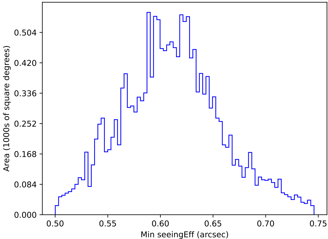
internal_u_expt38_nscale1.1v3.4_10yrs WFD r band: Min seeingEff
