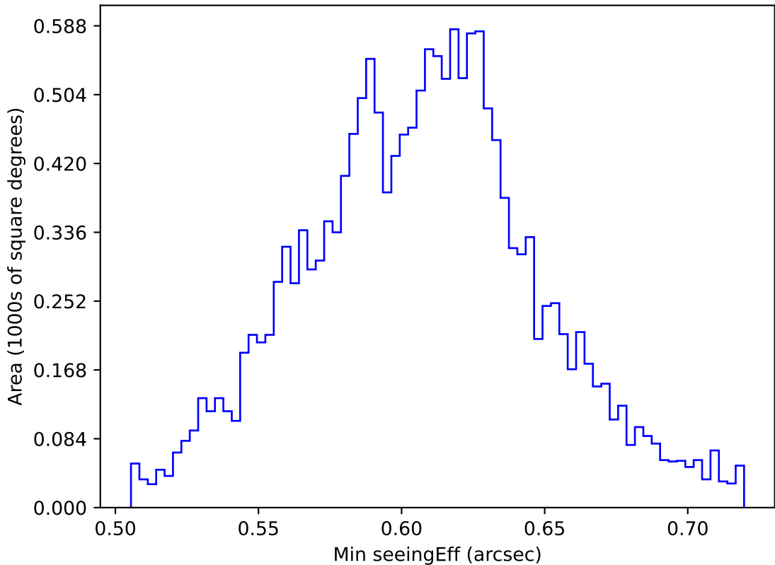
internal_u_expt38_nscale1.1v3.4_10yrs WFD i band: Min seeingEff
