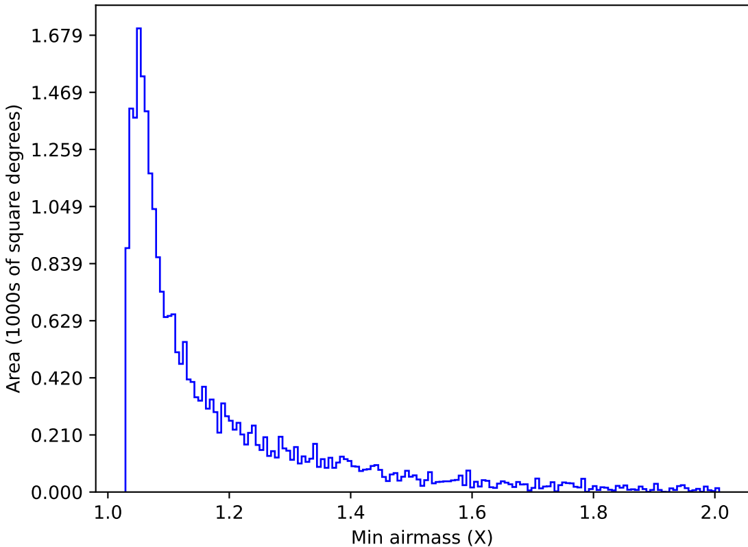
internal_u_expt38_nscale1.1v3.4_10yrs Yr 1 g band: Min airmass
