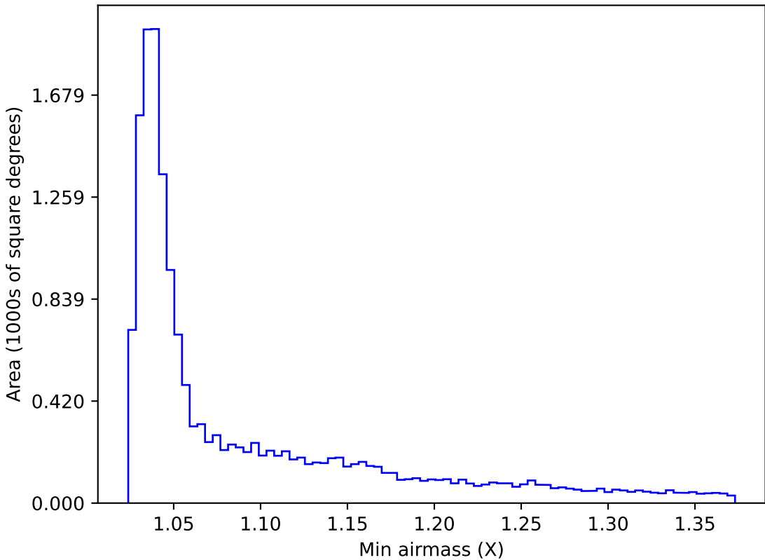
internal_u_expt38_nscale1.1v3.4_10yrs WFD u band: Min airmass
