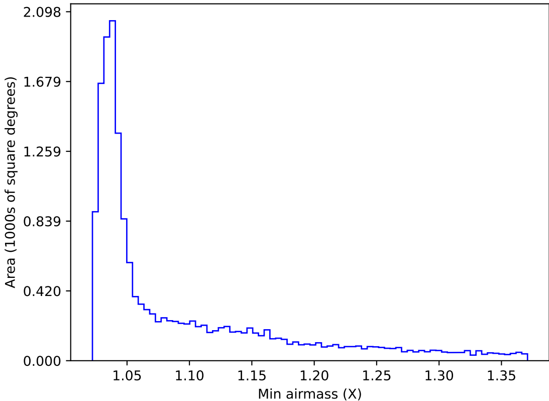
internal_u_expt38_nscale1.1v3.4_10yrs WFD g band: Min airmass
