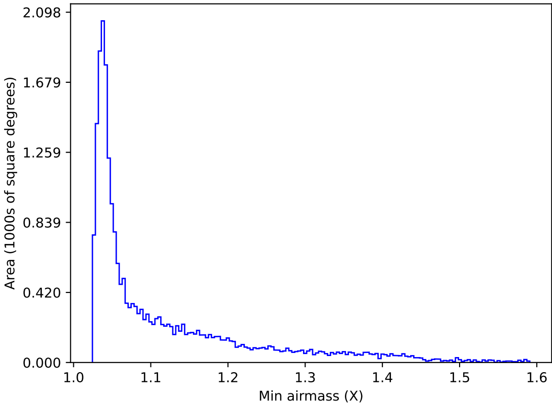
internal_u_expt38_nscale1.1v3.4_10yrs All sky u band: Min airmass
