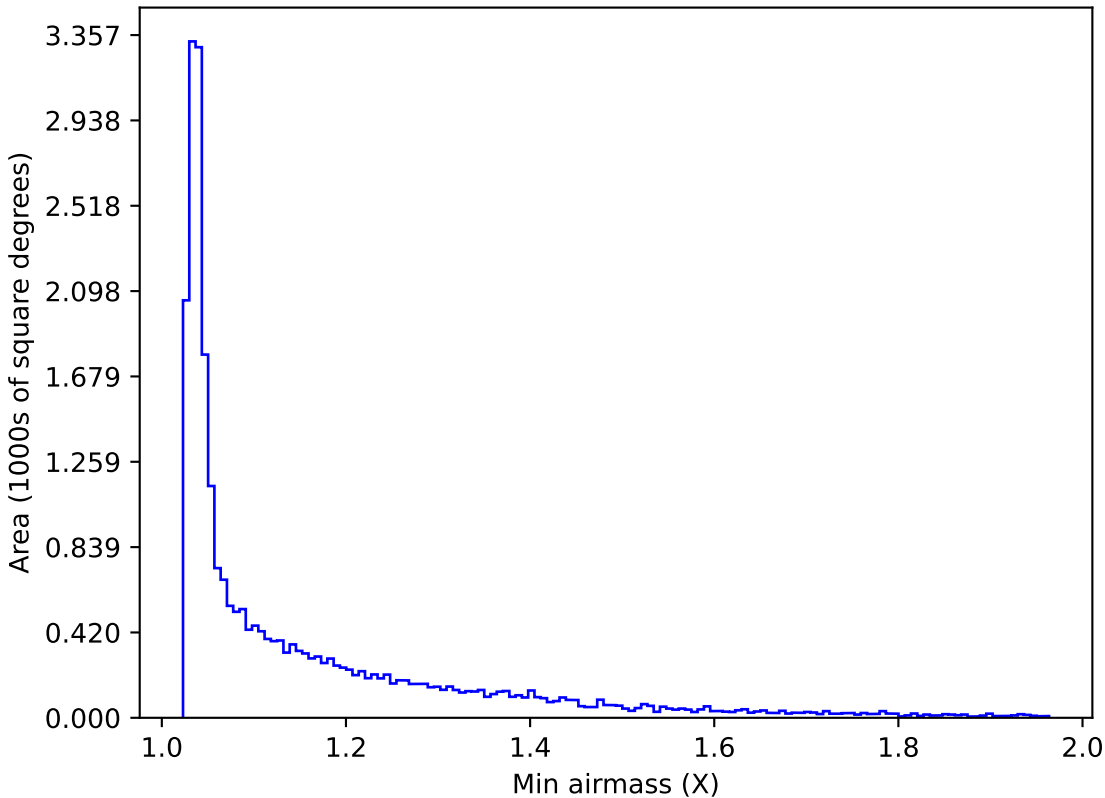
internal_u_expt38_nscale1.1v3.4_10yrs All sky g band: Min airmass
