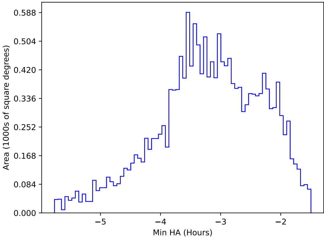
internal_u_expt38_nscale1.1v3.4_10yrs WFD u band: Min HA
