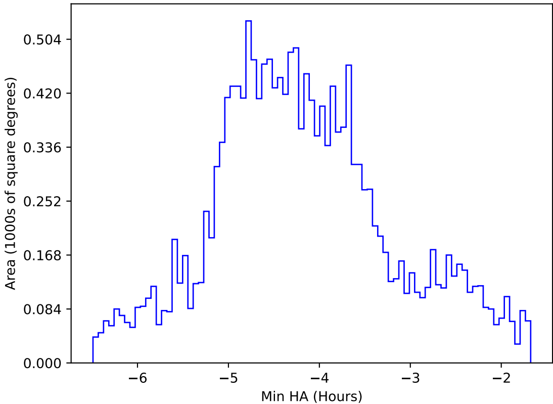
internal_u_expt38_nscale1.1v3.4_10yrs WFD g band: Min HA
