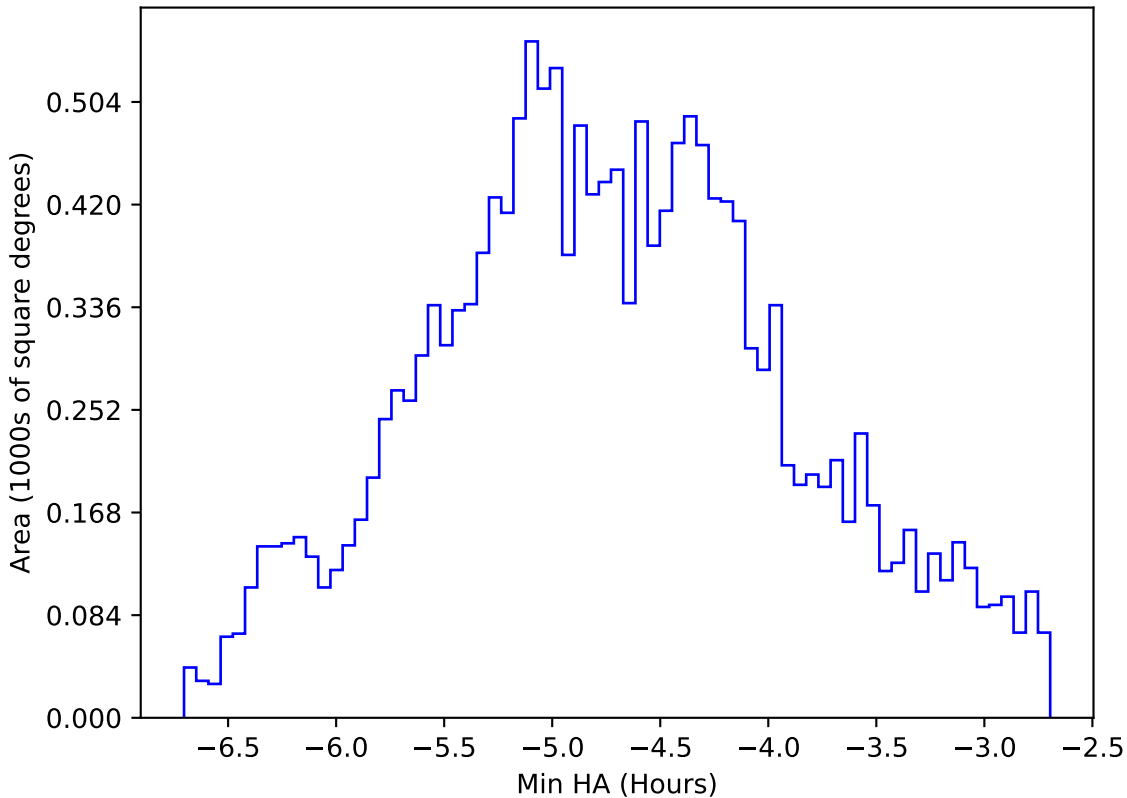
internal_u_expt38_nscale1.1v3.4_10yrs WFD all bands: Min HA
