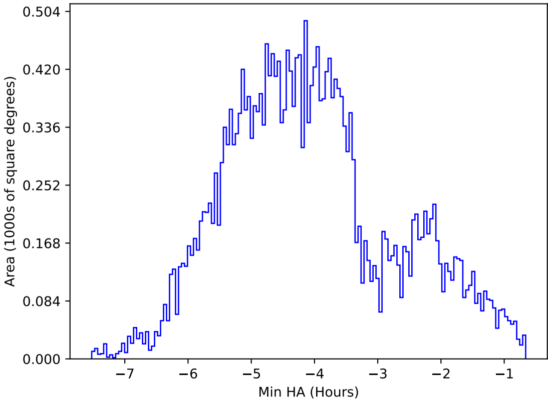
internal_u_expt38_nscale1.1v3.4_10yrs All sky z band: Min HA
