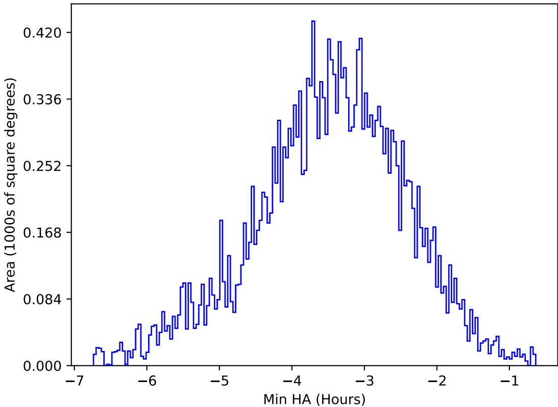
internal_u_expt38_nscale1.1v3.4_10yrs All sky y band: Min HA
