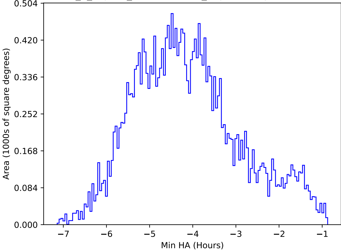
internal_u_expt38_nscale1.1v3.4_10yrs All sky r band: Min HA
