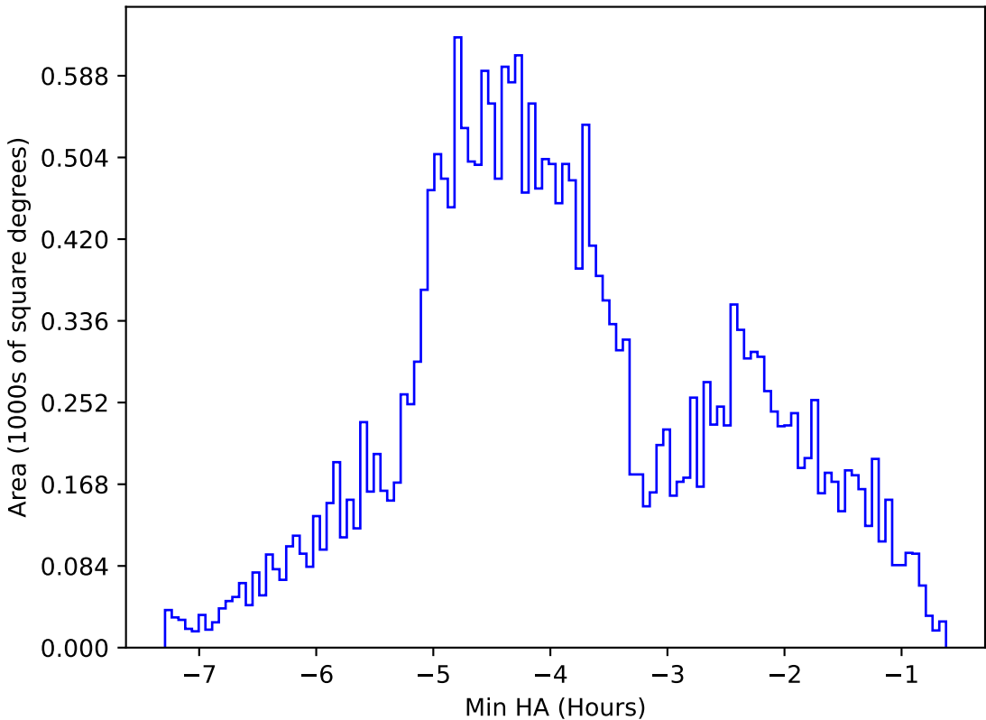
internal_u_expt38_nscale1.1v3.4_10yrs All sky g band: Min HA
