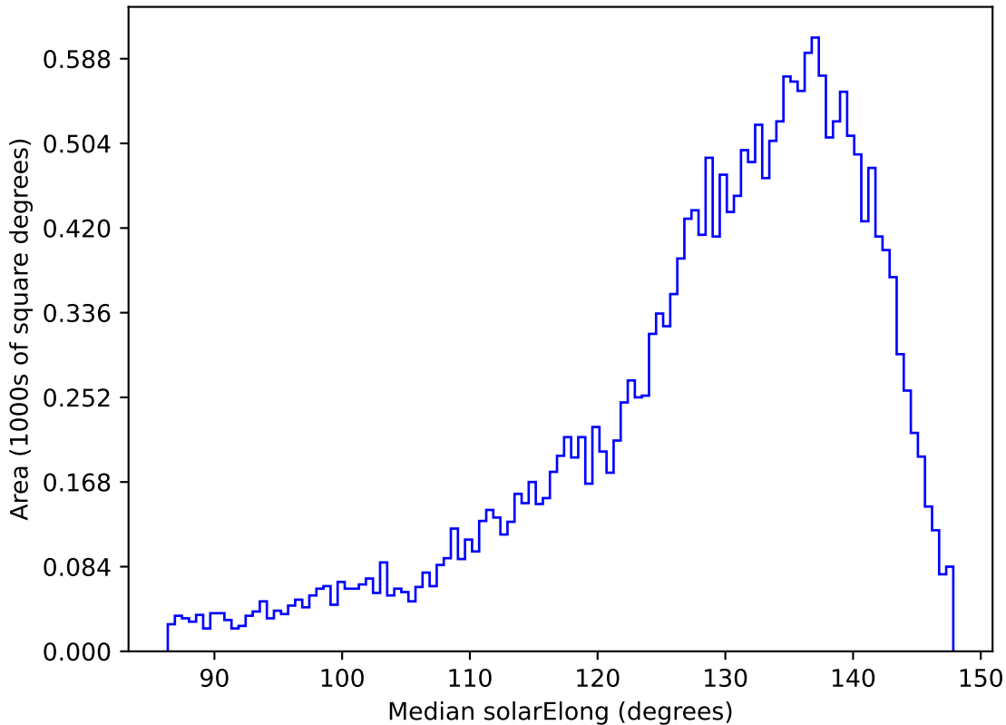
internal_u_expt38_nscale1.1v3.4_10yrs All sky y band: Median solarElong
