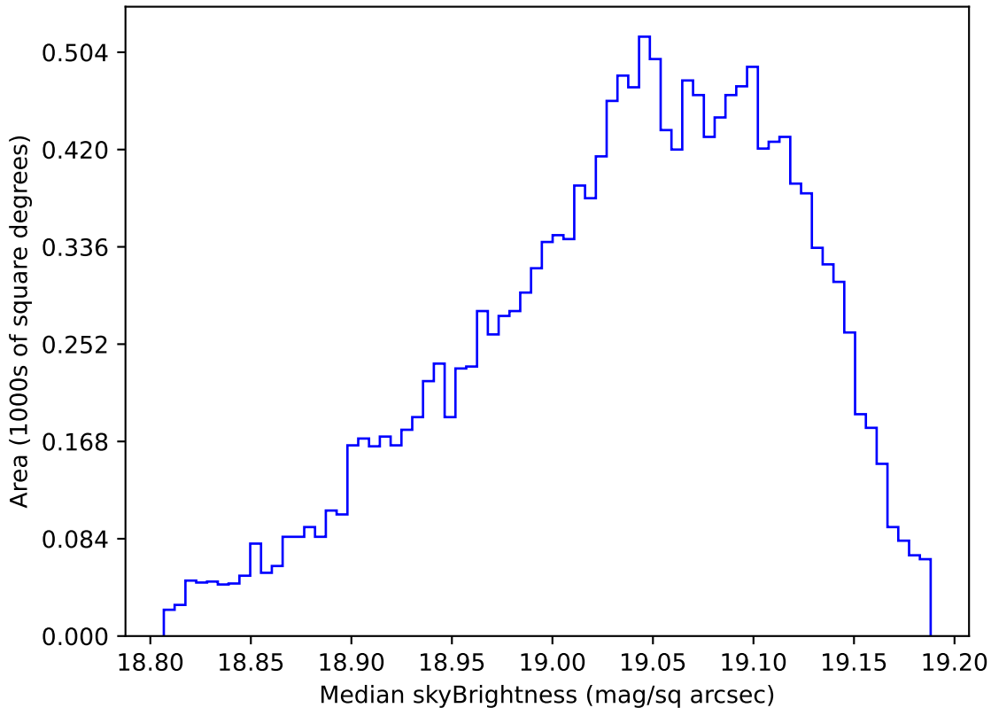
internal_u_expt38_nscale1.1v3.4_10yrs WFD z band: Median skyBrightness
