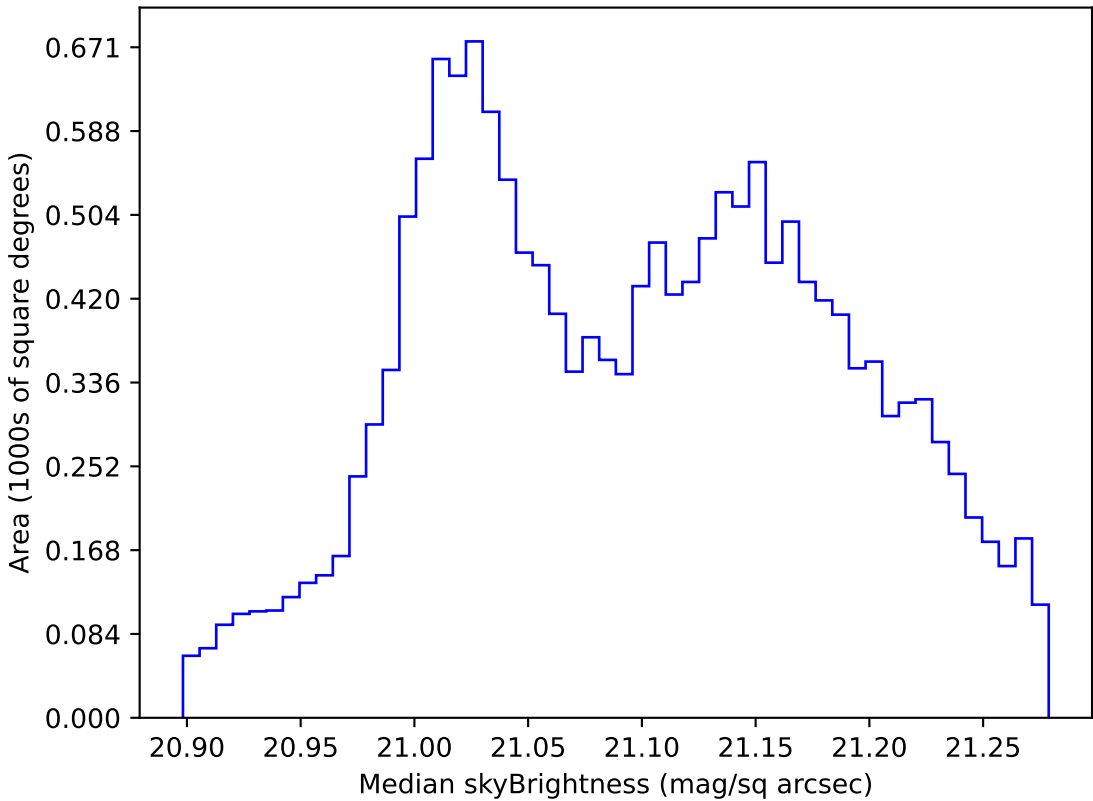
internal_u_expt38_nscale1.1v3.4_10yrs WFD r band: Median skyBrightness
