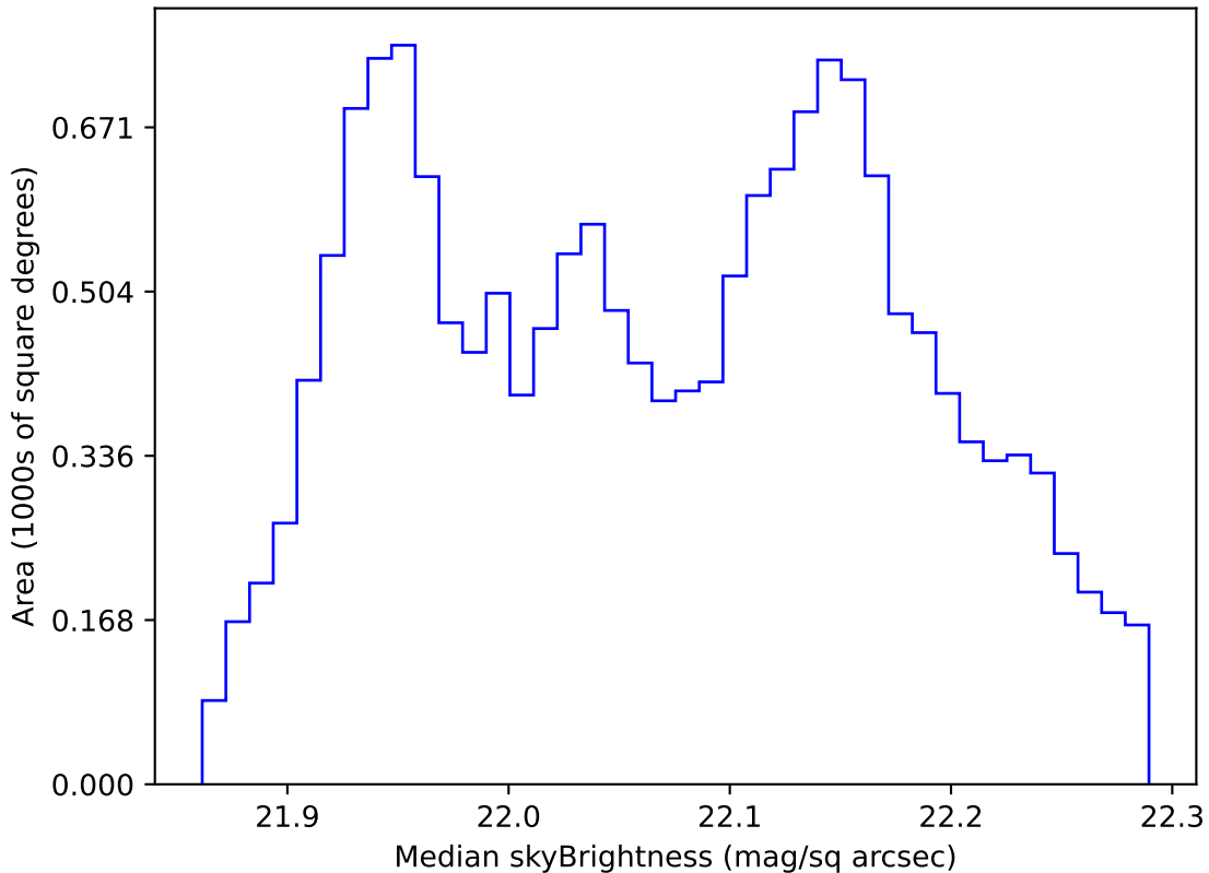
internal_u_expt38_nscale1.1v3.4_10yrs WFD g band: Median skyBrightness
