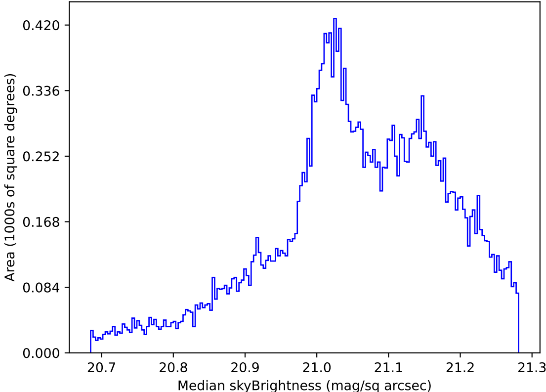
internal_u_expt38_nscale1.1v3.4_10yrs All sky r band: Median skyBrightness
