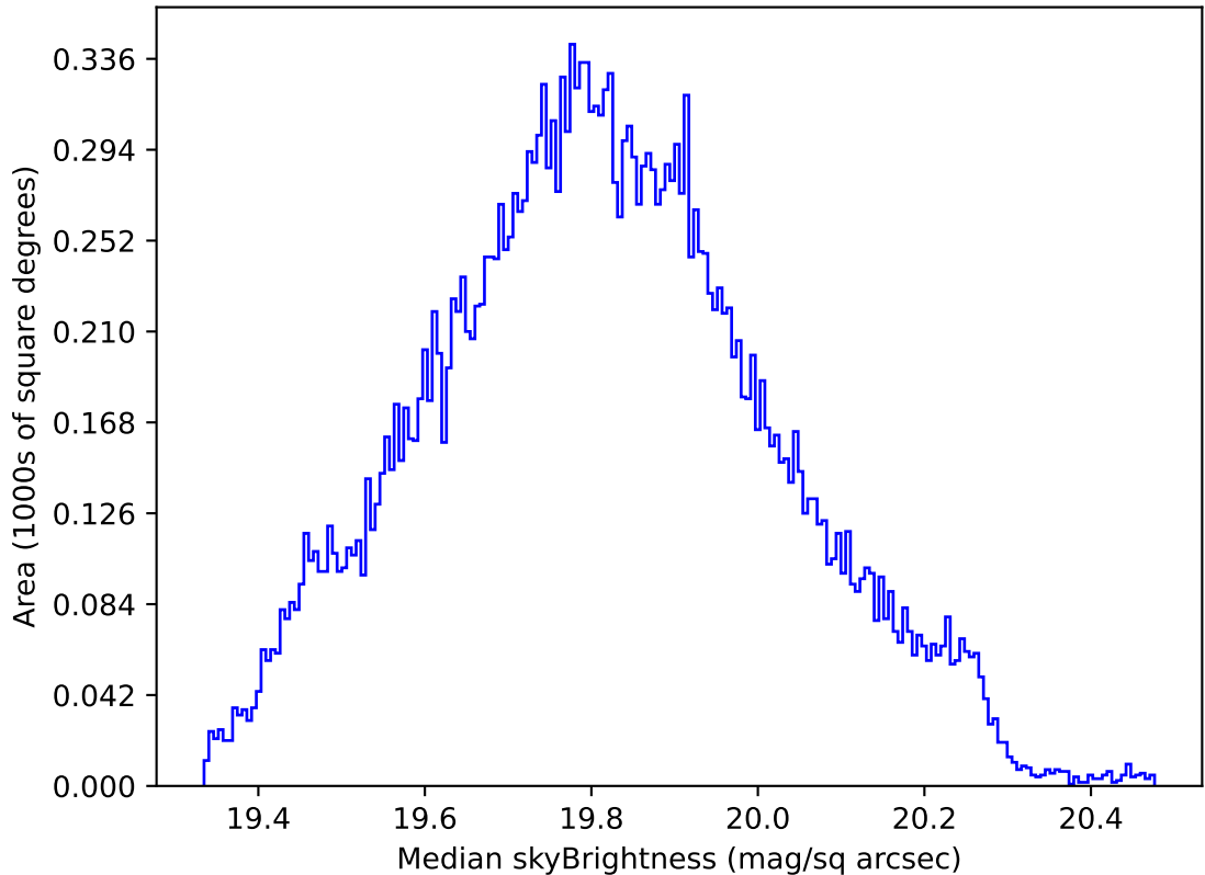
internal_u_expt38_nscale1.1v3.4_10yrs All sky all bands: Median skyBrightness
