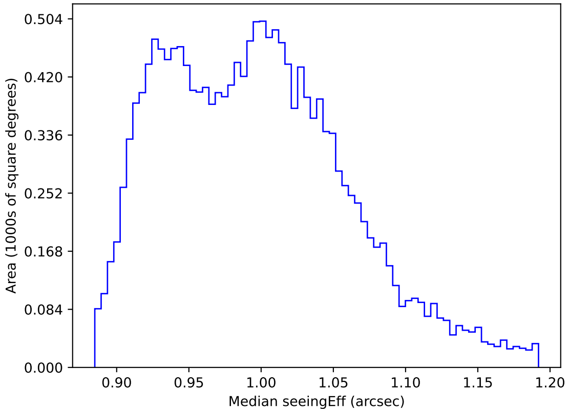
internal_u_expt38_nscale1.1v3.4_10yrs WFD y band: Median seeingEff
