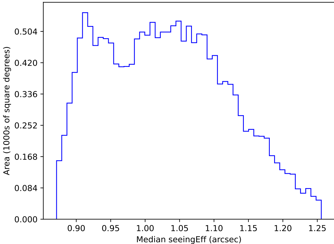
internal_u_expt38_nscale1.1v3.4_10yrs WFD r band: Median seeingEff
