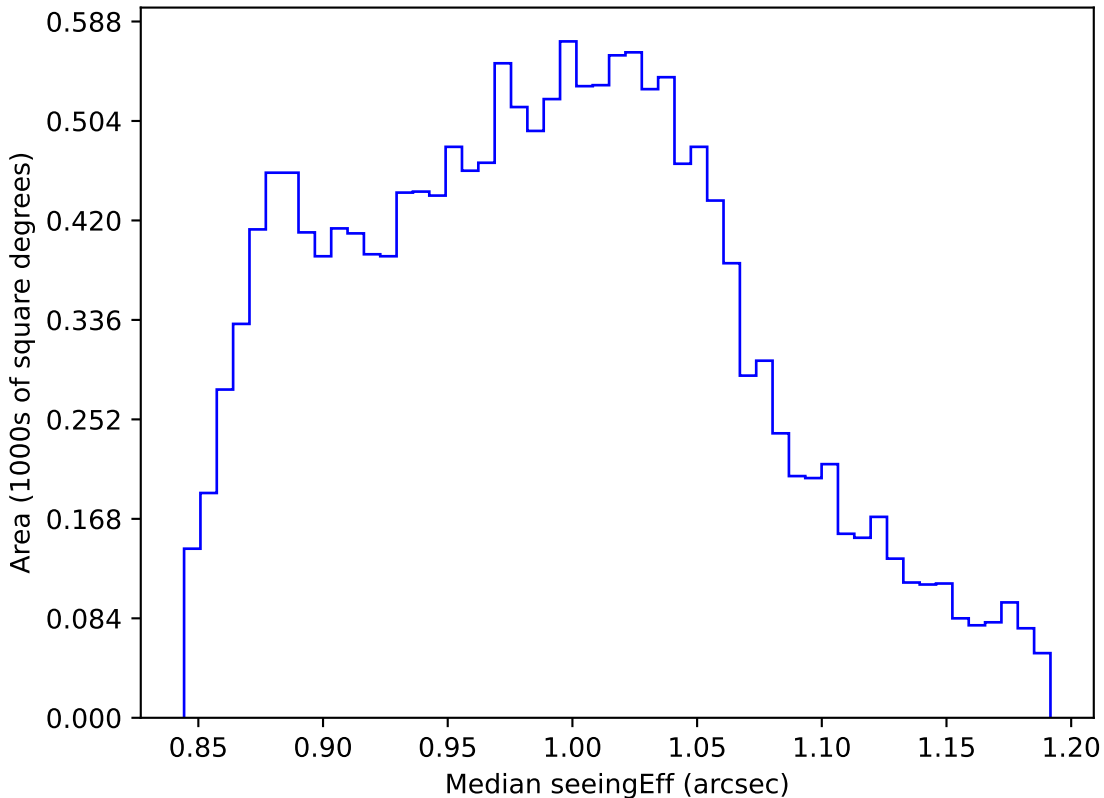
internal_u_expt38_nscale1.1v3.4_10yrs WFD i band: Median seeingEff
