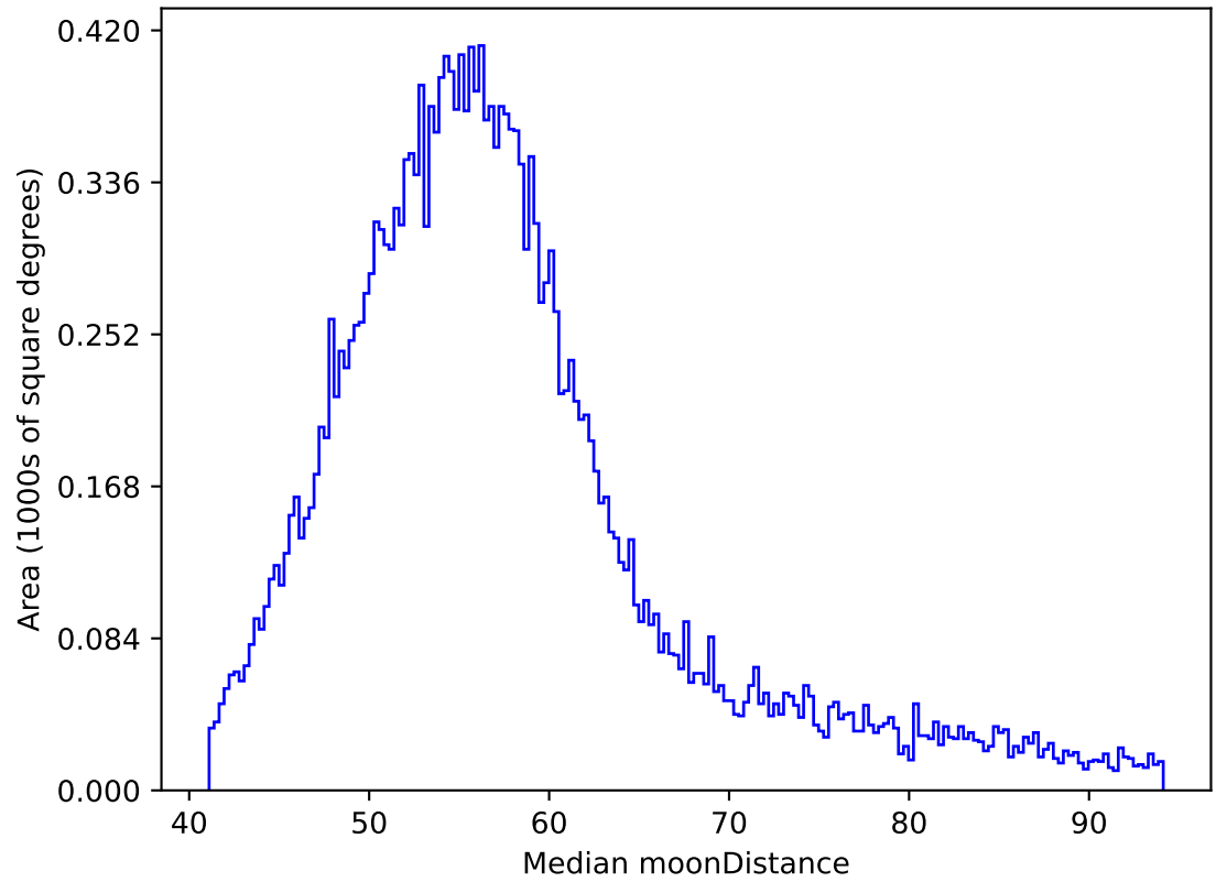
internal_u_expt38_nscale1.1v3.4_10yrs All sky y band: Median moonDistance
