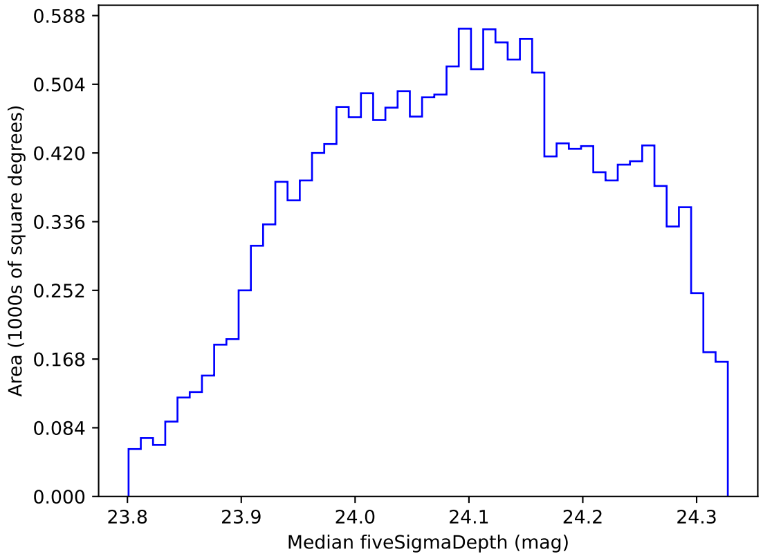
internal_u_expt38_nscale1.1v3.4_10yrs WFD r band: Median fiveSigmaDepth
