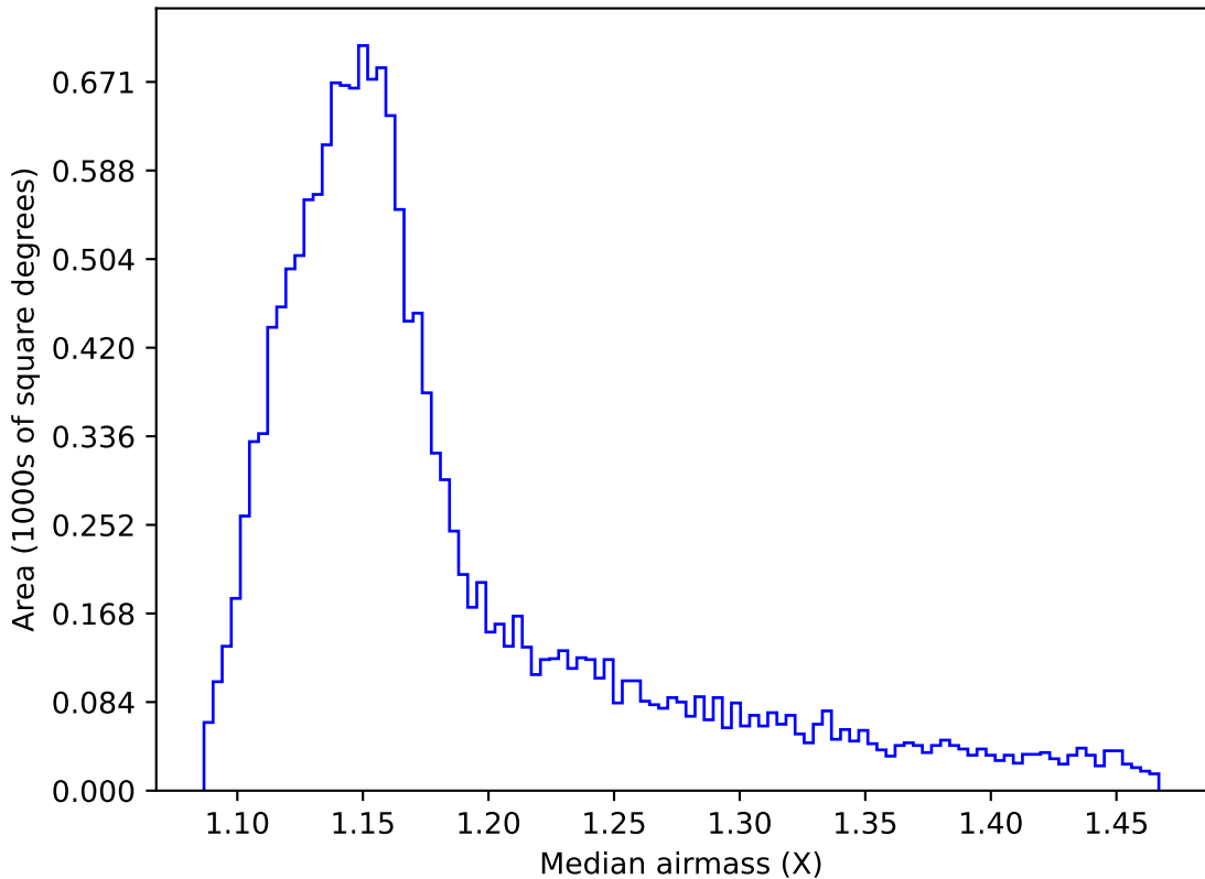
internal_u_expt38_nscale1.1v3.4_10yrs WFD z band: Median airmass
