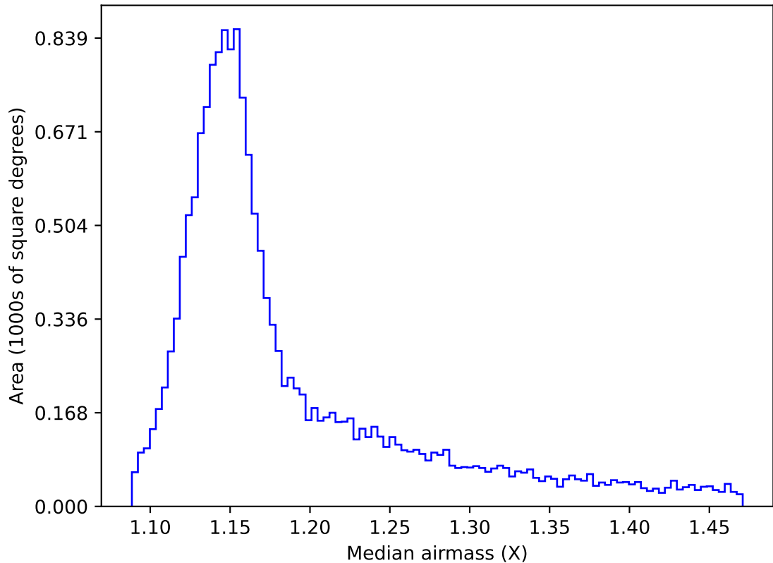
internal_u_expt38_nscale1.1v3.4_10yrs WFD y band: Median airmass
