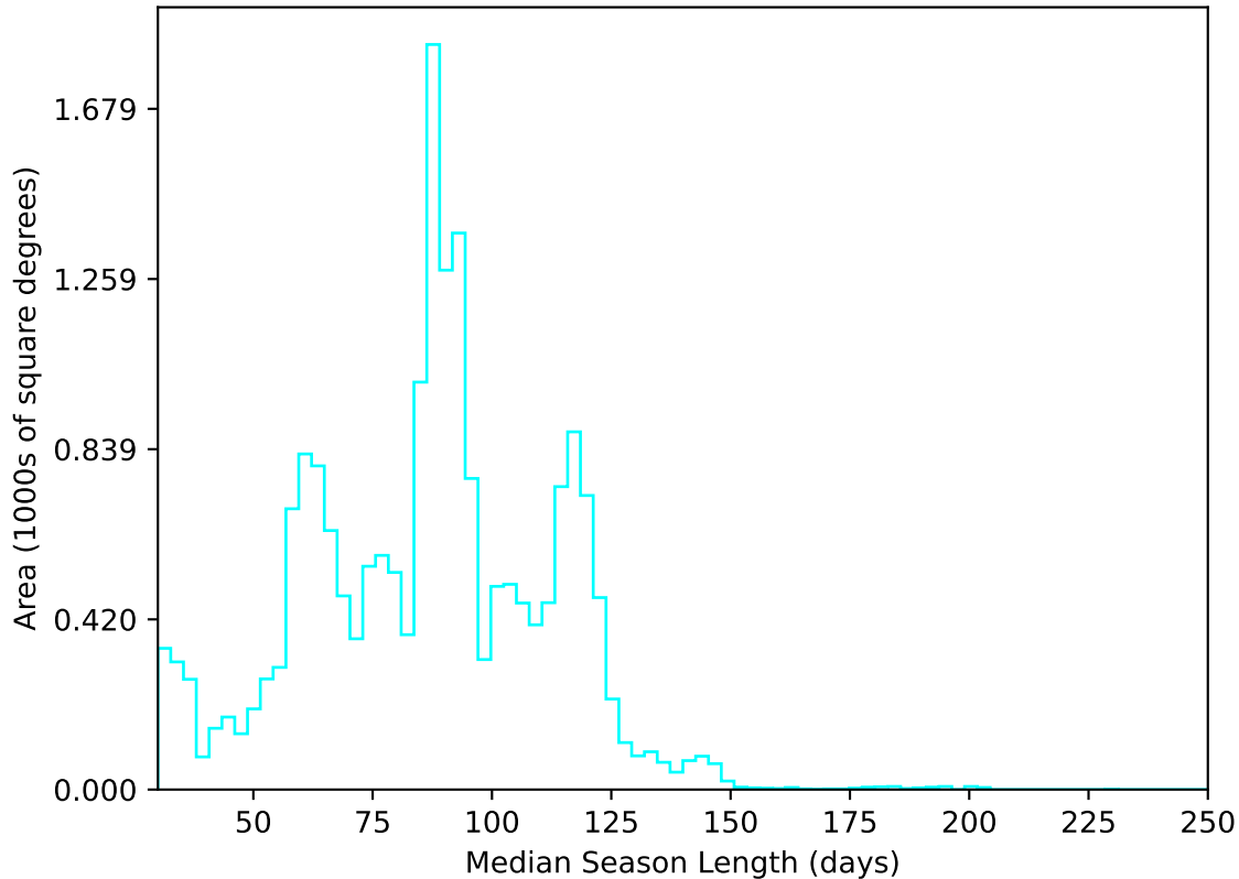
internal_u_expt38_nscale1.1v3.4_10yrs All sky u band: Median Season Length
