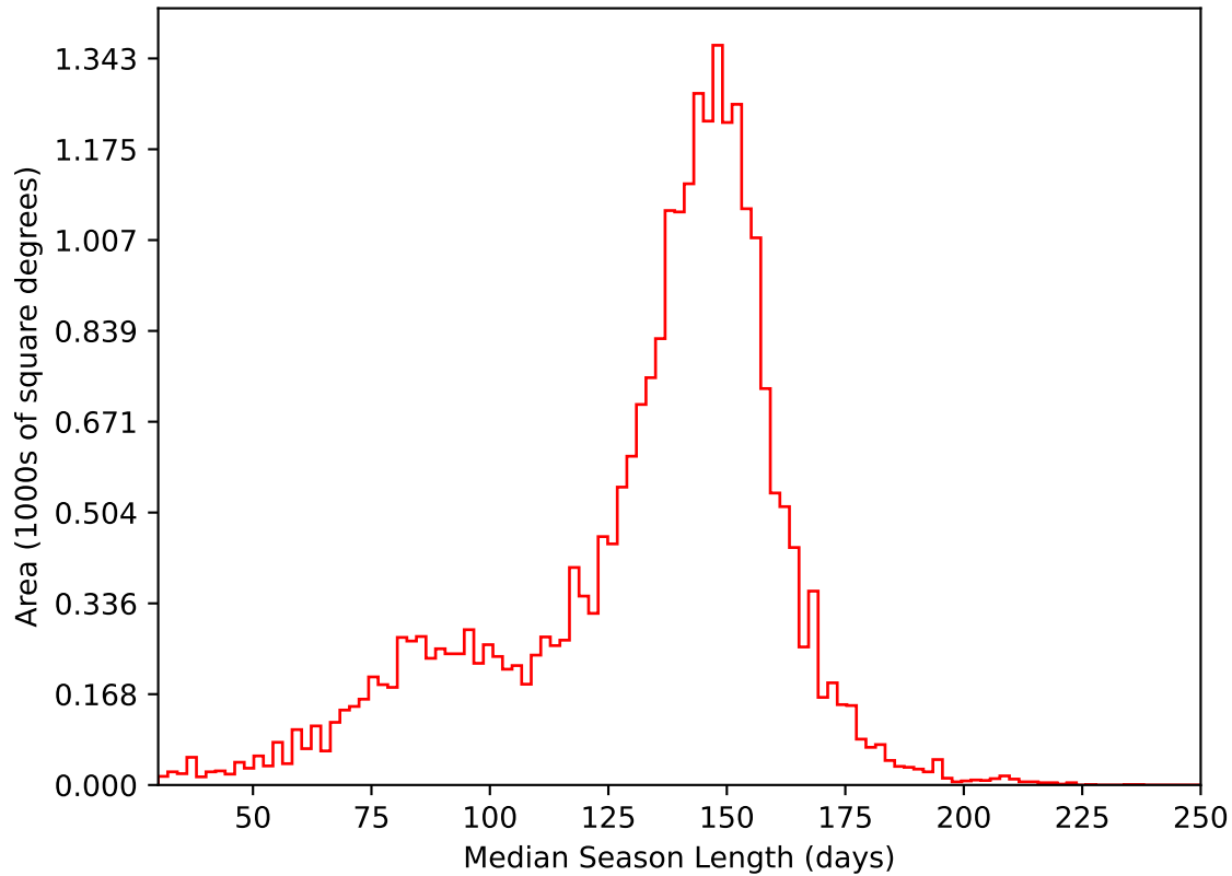
internal_u_expt38_nscale1.1v3.4_10yrs All sky i band: Median Season Length
