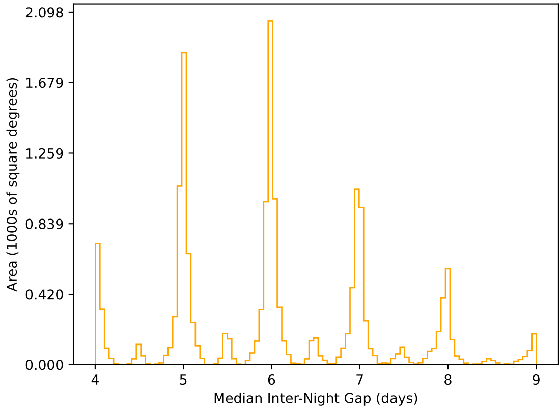
internal_u_expt38_nscale1.1v3.4_10yrs WFD r band: Median Inter-Night Gap
