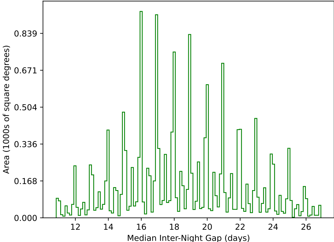
internal_u_expt38_nscale1.1v3.4_10yrs WFD g band: Median Inter-Night Gap
