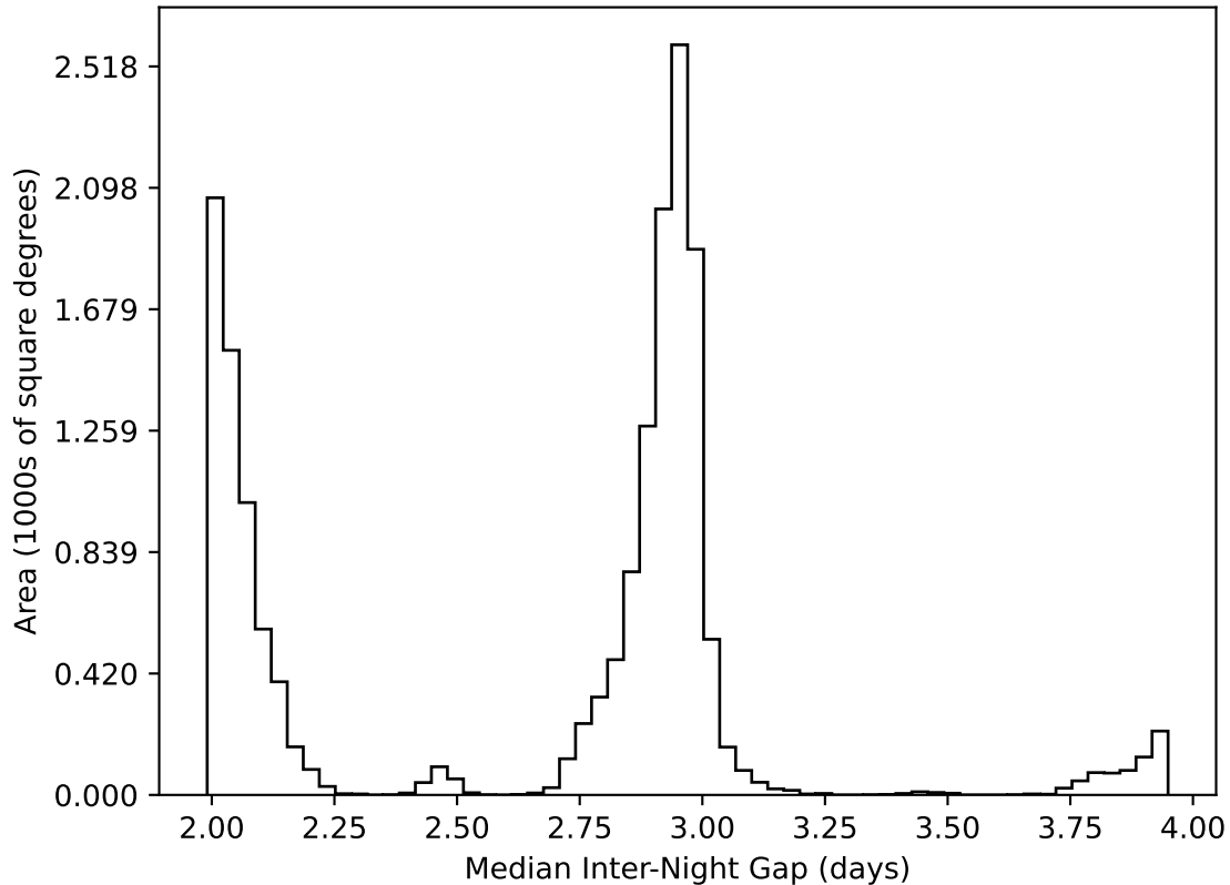
internal_u_expt38_nscale1.1v3.4_10yrs WFD all bands: Median Inter-Night Gap
