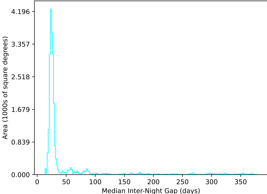
internal_u_expt38_nscale1.1v3.4_10yrs All sky u band: Median Inter-Night Gap
