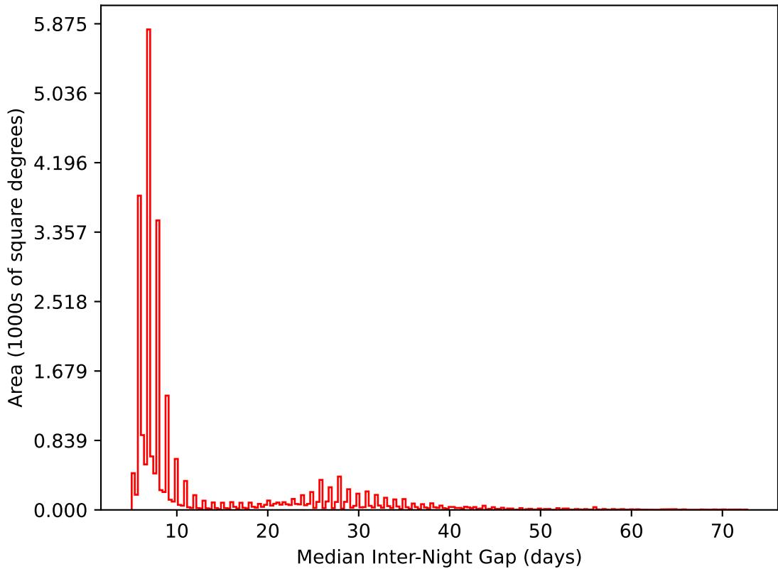
internal_u_expt38_nscale1.1v3.4_10yrs All sky i band: Median Inter-Night Gap
