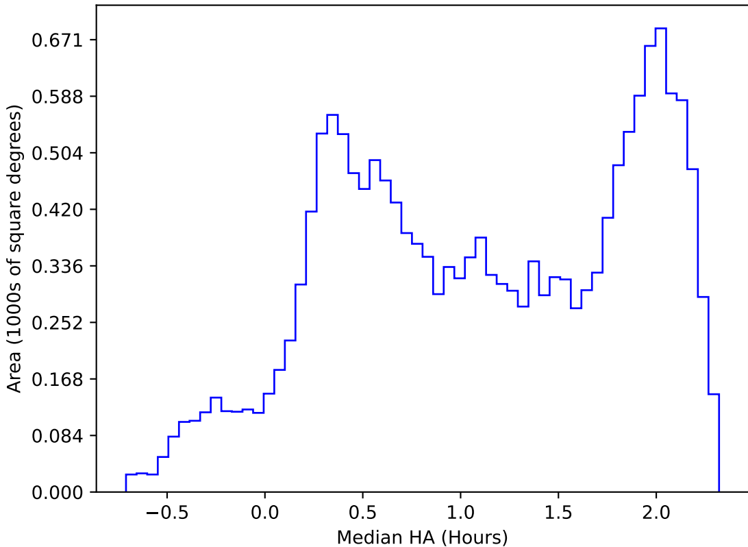
internal_u_expt38_nscale1.1v3.4_10yrs WFD z band: Median HA
